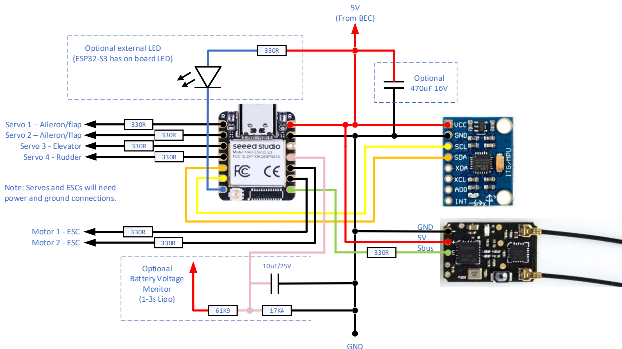
Figure 1 – 5V Wiring Diagram
