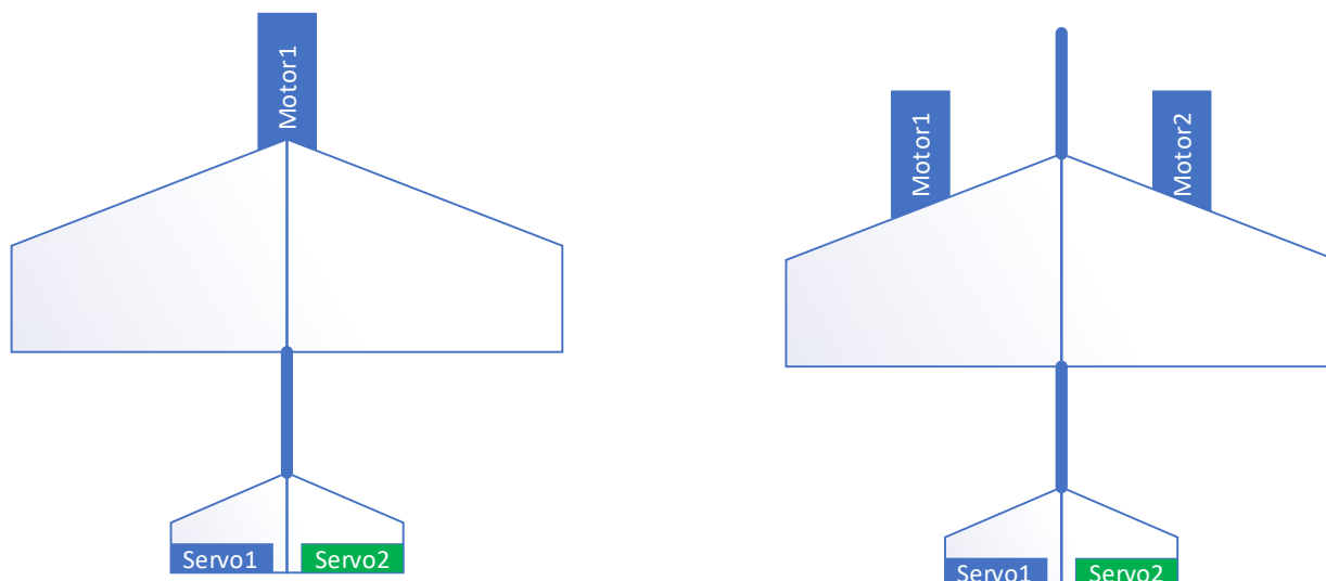
Figure 17 - PLANE_V_TAIL
